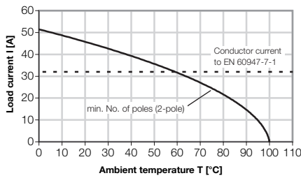
TOP 4GS 7.62/90 / H07V-K4.0
